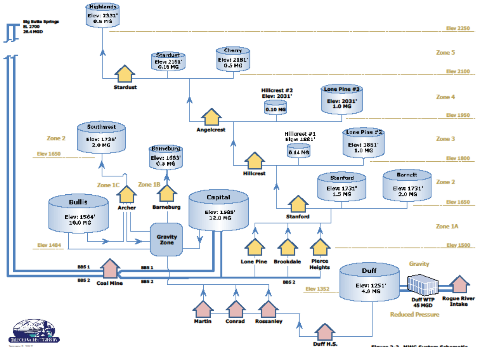
Figure 2-2. MWC System Schematic
